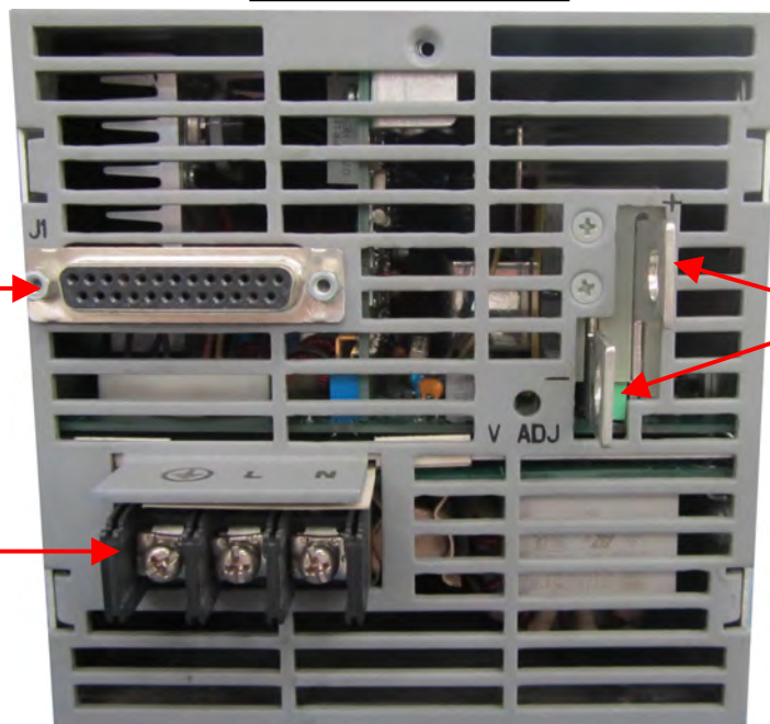
IO Connections
